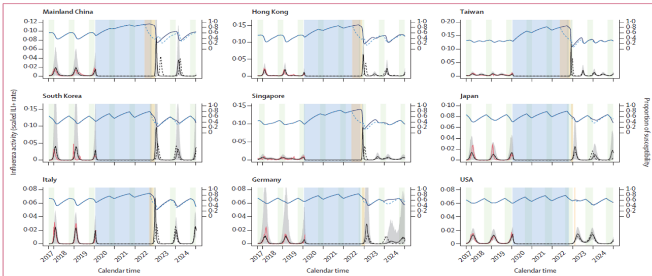
Figure 4: Prediction of upcoming influenza activity when COVID-19 PHSMs are relaxed in October, 2022, (before the winter season) with proactive vaccination programmes (one-off vaccination timing, duration, and rate) to mitigate the excess influenza activity in nine locations and countries
